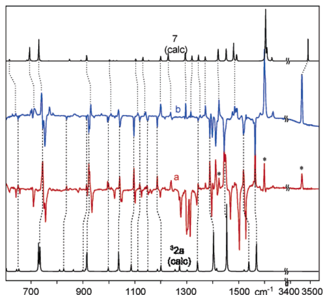
Figure 2. IR difference spectra for (a) the formation (254-nm photolysis of azide 1a , red spectrum) and (b) the >515-nm bleaching (blue spectrum) of nitrene 32a in an Ar matrix at 12 K. The bands that increase in a and decrease in b (dashed lines) are correlated with those of the simulated spectrum of nitrene 32a at the bottom (B3LYP/6-31G* calculation of most stable conformer). The bands that increase in spectrum b are correlated with those of the simulated spectrum of pyrazoloindole 7 shown at the top (dotted lines).
