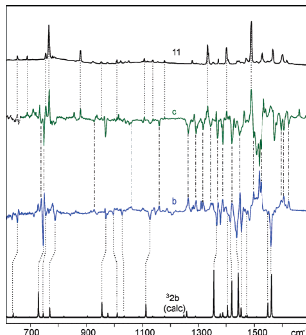
Figure 4. IR difference spectra corresponding to spectra b (blue line) and c (green line) in Figure 3. The bands that decrease in b are correlated with those of the simulated spectrum of nitrene ^3\mathbf{2b} . (B3LYP/6-31G* calculation of most stable conformer) at the bottom. Peaks that rise in b and decrease in c (dashend lines) are due to dihydroquinoxaline 8 , while those that rise in c are correlated with the IR spectrum of quinoxaline 11 at the top.
